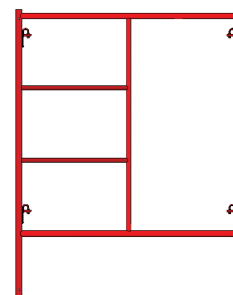
B-FS5W67H-D48 5'x6'7" Step Frame 1.625", D-Lk 48" Spacing 47.9 lbs.
