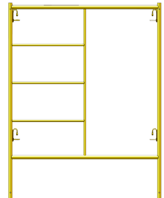
BKF5567D48 B-Size Step Frame 5'x6'7" 48.27 lbs.
